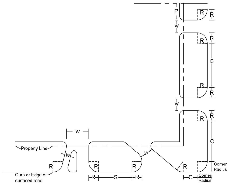
(1) Figure 2. Driveway Dimension Measurements (See Table 7)
