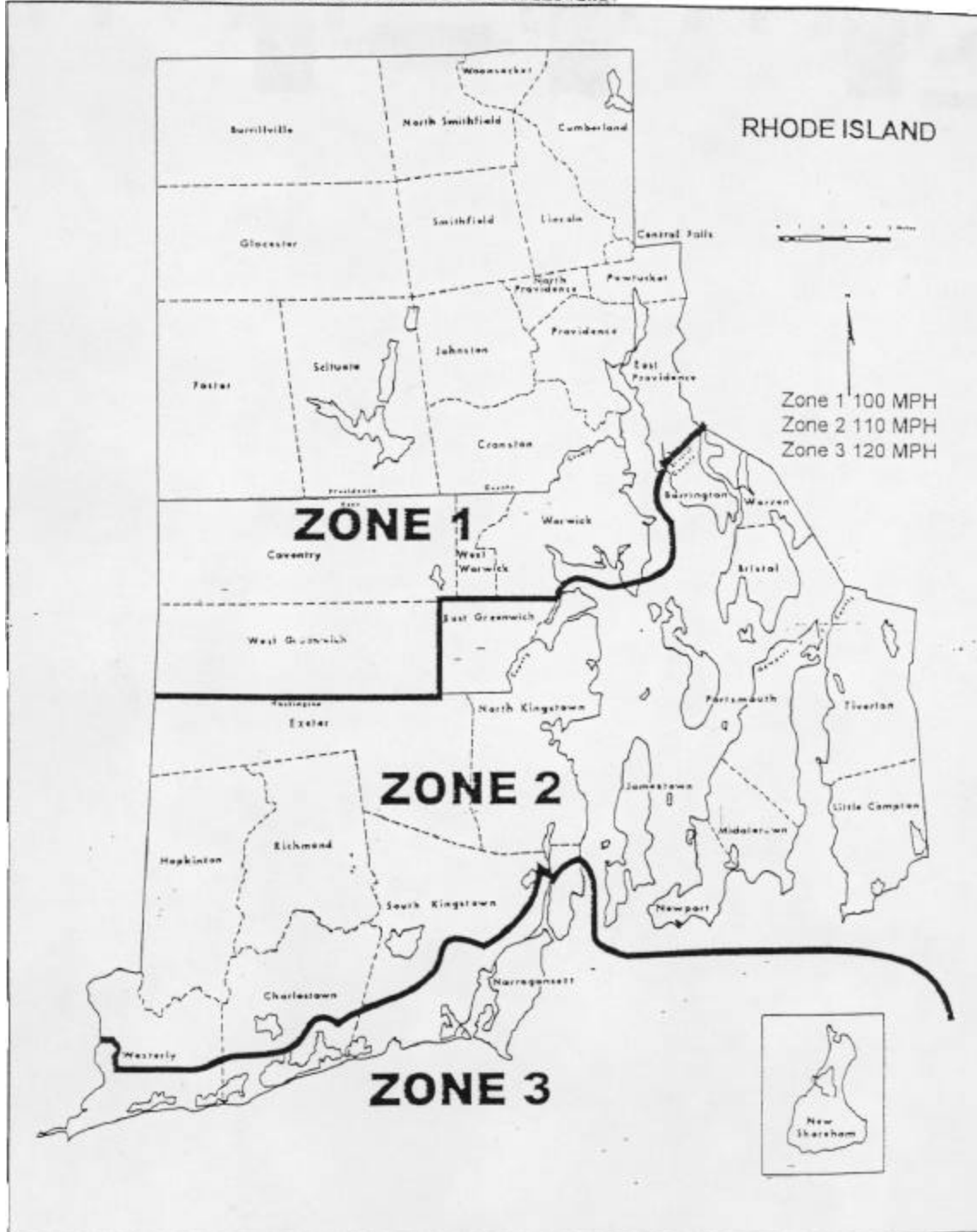
FIGURE 1609
