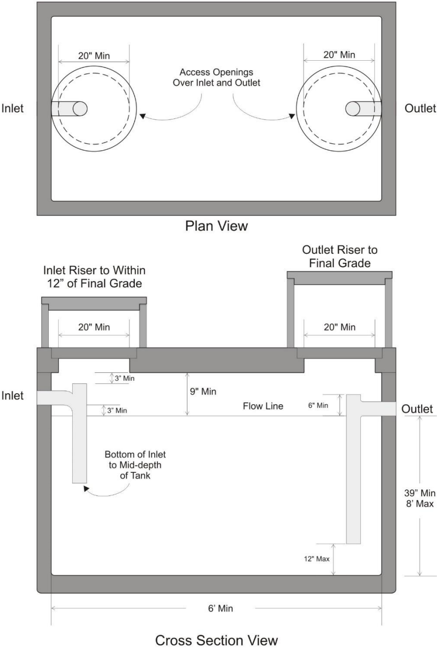
Figure 4: Grease Tanks Not To Scale, Consult § 6.26 of this Part For Details
