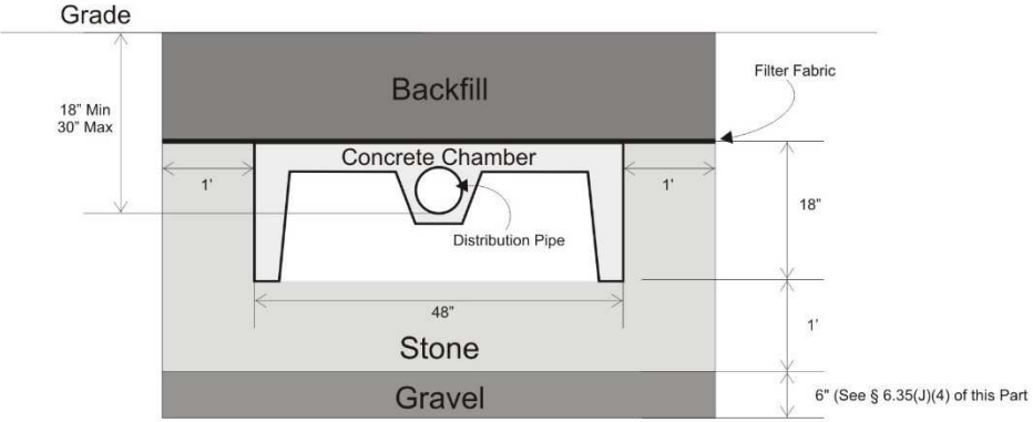
Typical Trench Cross Section View
