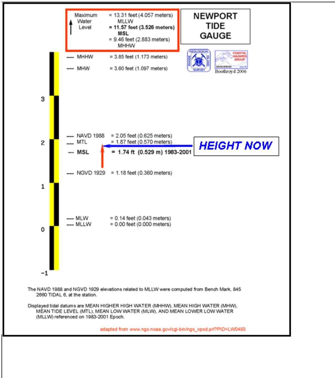
Figure 6: Comparison of tidal and fixed vertical datums at the Newport Tide Gauge. (Boothroyd, 2007).
