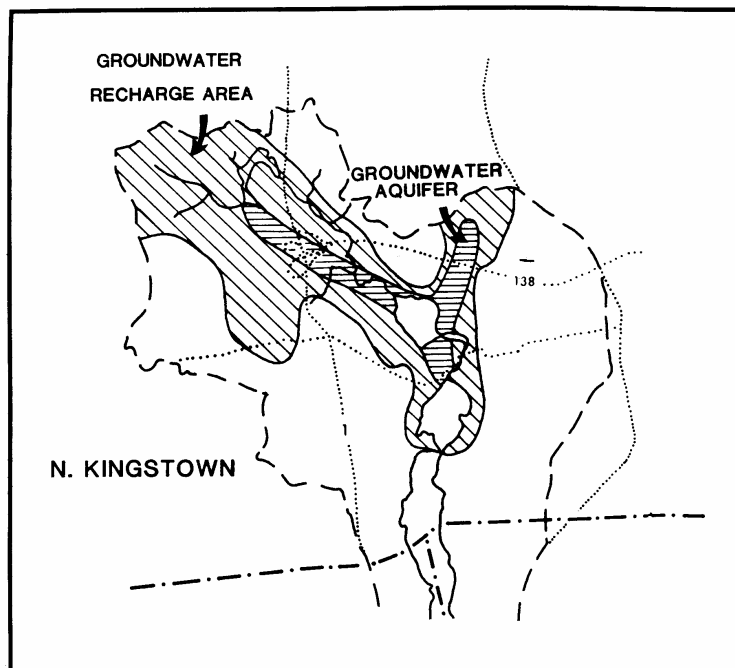
Figure 3-22. Location of aquifer and groundwater recharge zone.
