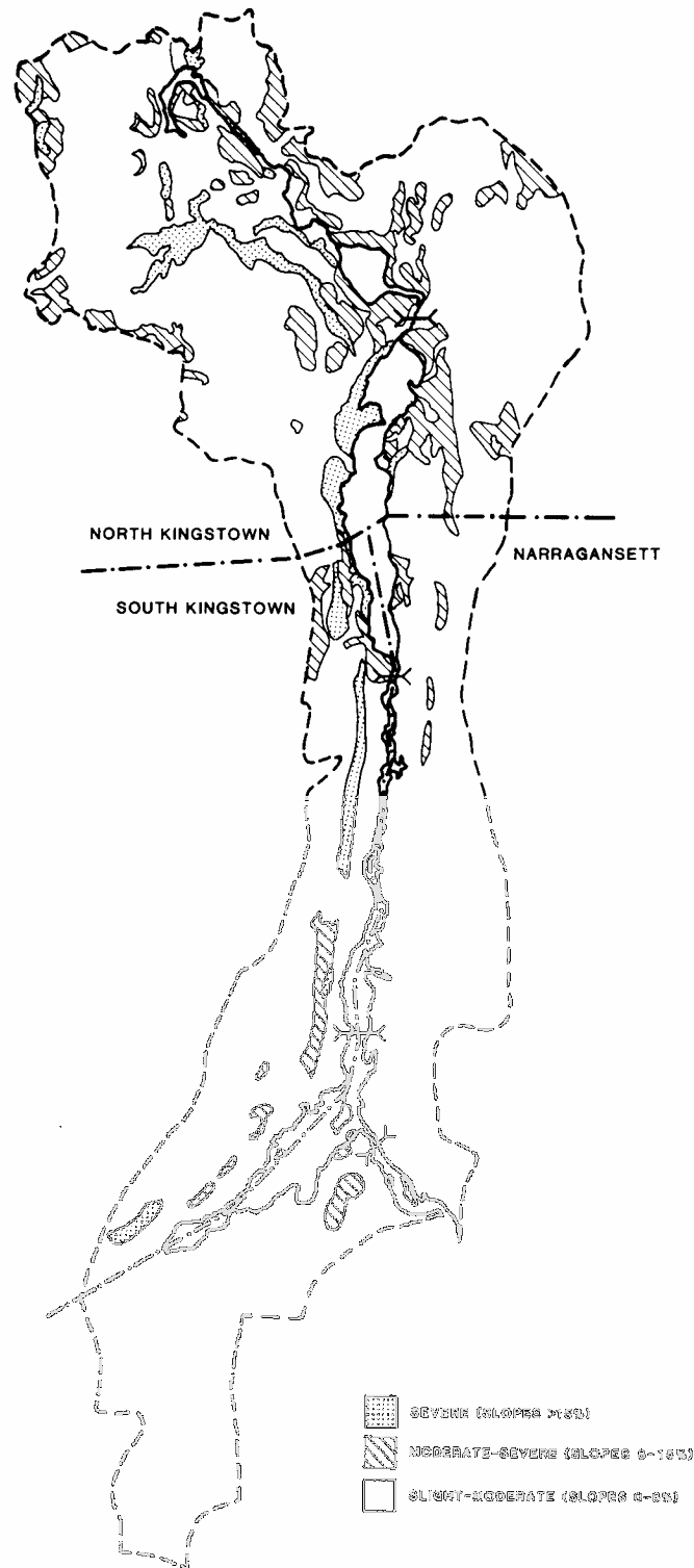
Figure 3-13. Erosion Potential
