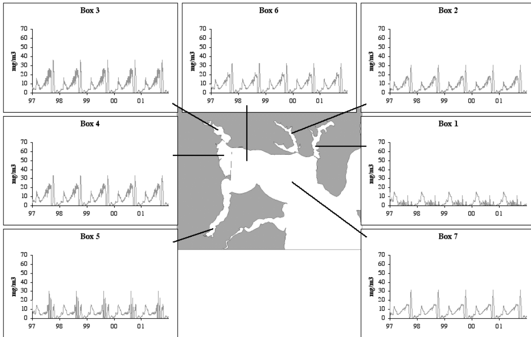
Fig. 14. Concentrations of surface chlorophyll-a from the 5-year simulation under pre-colonial conditions.
