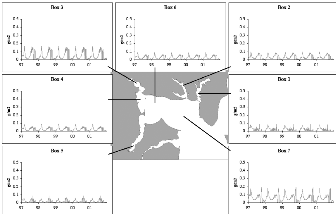
Fig. 16. As in Fig. 14, but for bottom layer sediment carbon concentrations.
