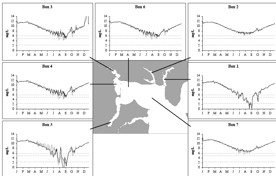
Fig. 6. As in Fig. 5, but for bottom O 2 concentrations.
