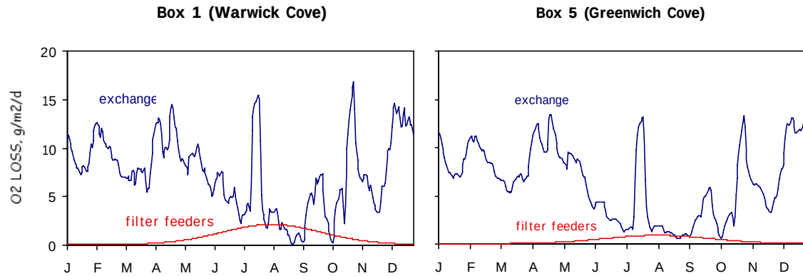
Fig. 3. Modeled oxygen losses due to water exchange (physical circulation) and filter feeders in a model run without primary producers. Other losses were insignificant.
