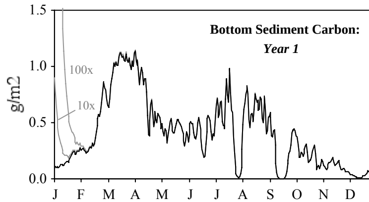
Fig. 13. Predicted sediment carbon concentrations in Greenwich Cove from the first year of the 5-year run under current conditions and using 1, 10, and 100x the initial concentrations from the standard run (black line).
