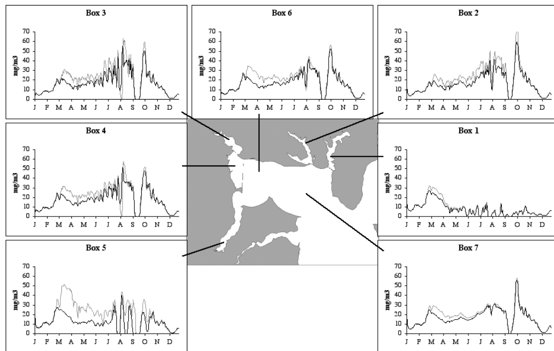
Fig. 7. Concentrations of surface chlorophyll-a with pre-colonial watershed inputs (black) compared to the standard run (grey).
