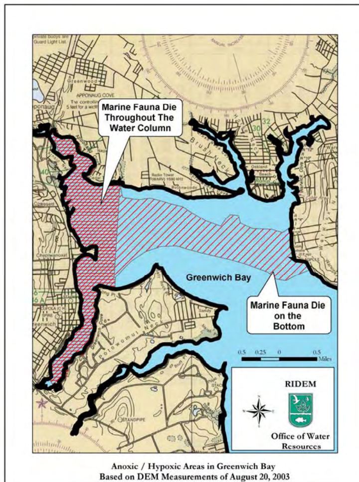
Figure 18. Hypoxic and anoxic areas in Greenwich Bay based on RIDEM measurements of August 20, 2003
