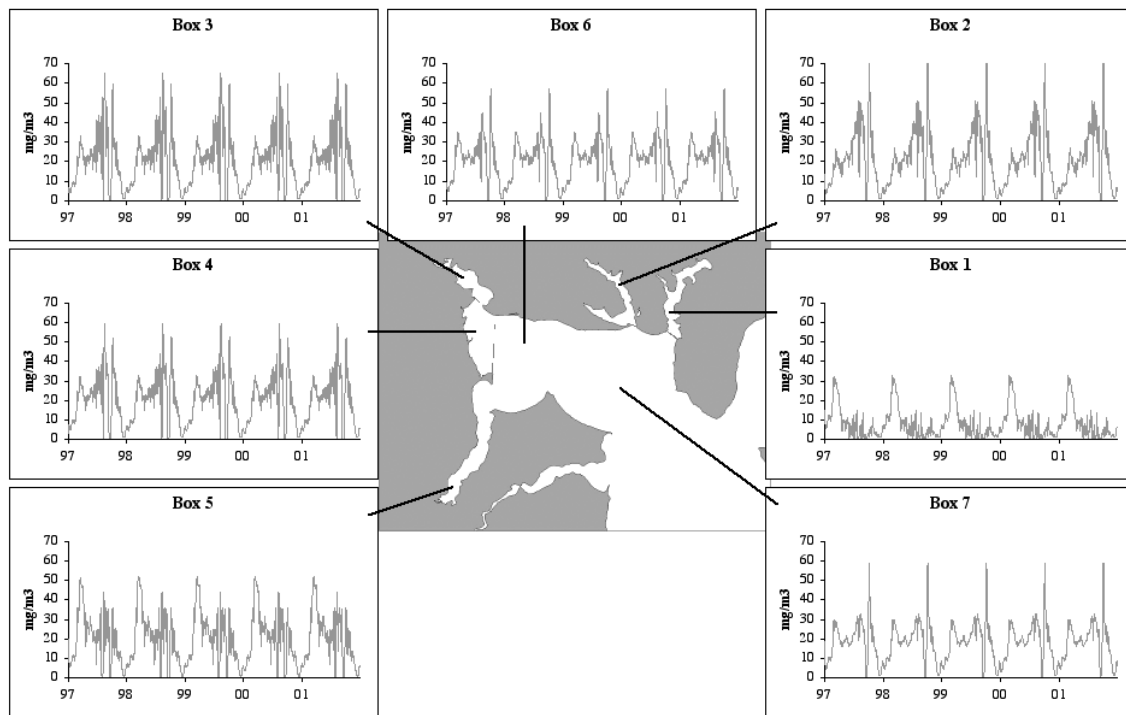
Fig. 9. Concentrations of surface chlorophyll- a from the 5-year simulation under current conditions.
