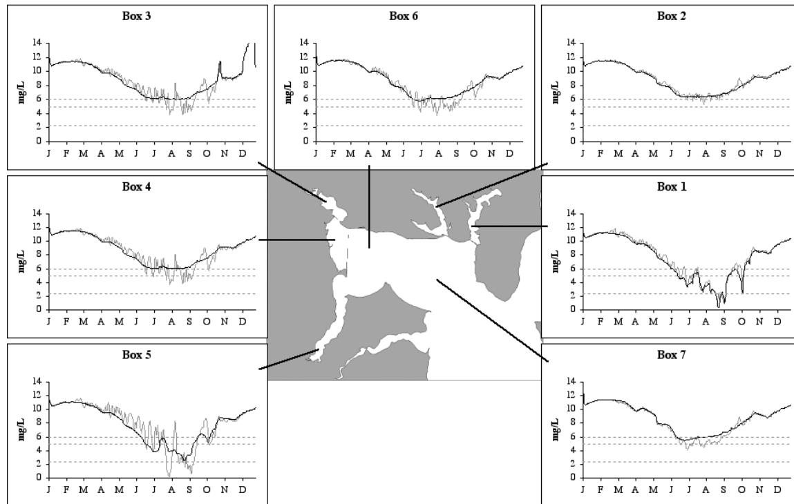
Fig. 2. Modeled concentrations of bottom water dissolved oxygen in a run without primary producers (black line) compared to the standard model run (grey line). In this and all figures, the horizontal dashed lines represent reference oxygen concentrations of 2.3, 5, and 6 mg/L.
