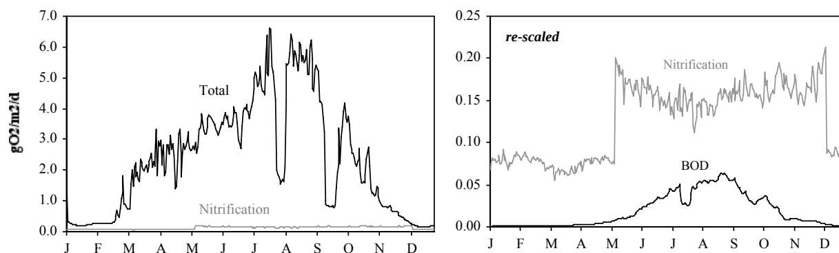
Fig. 1. Oxygen demand in Greenwich Cove due to nitrification of treatment plant ammonia compared with other sinks. The panel to the right is re-scaled to compare the demands due to nitrification and plant BOD.
